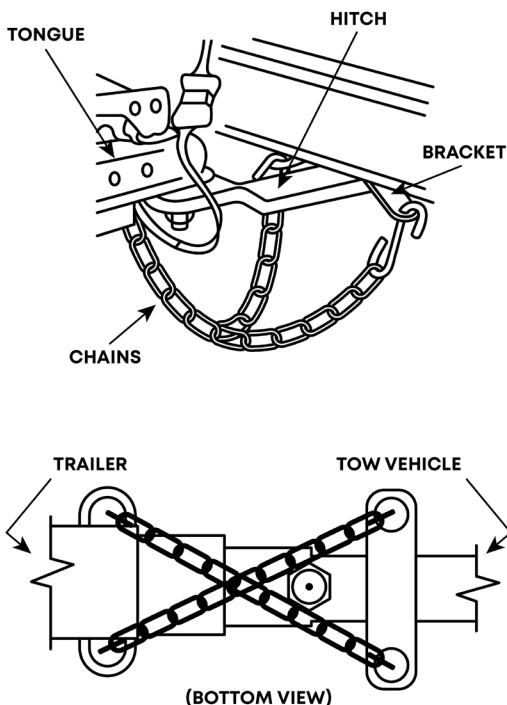
FIGURE 4-1 SAFETY CHAINS
