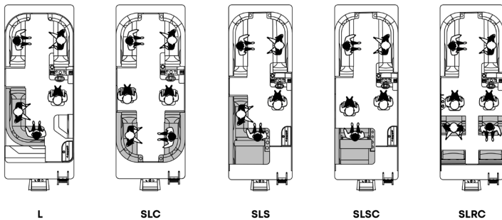
FIGURE 5-1 SEATING EVEN WEIGHT DISTRIBUTION FOR FLOORPLANS
