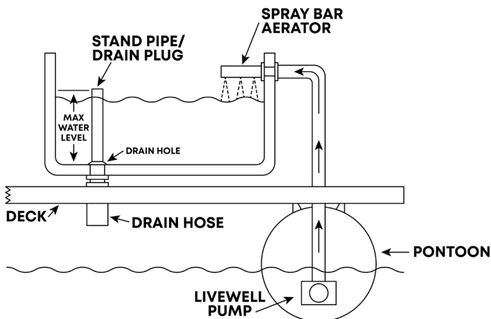
FIGURE 3-1 TYPICAL LIVEWELL
