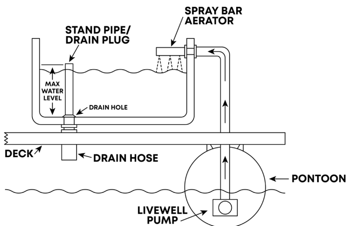
FIGURE 3-1 TYPICAL LIVEWELL
