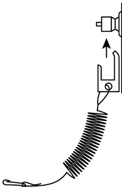
FIGURE 2-10 LANYARD STOP SWITCH
