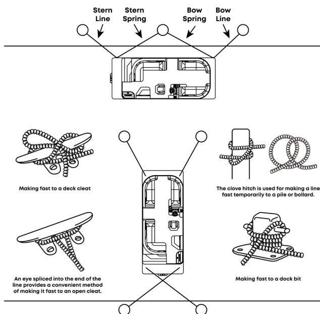
FIGURE 5-5 MOORING
