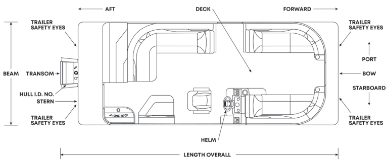
FIGURE 1-1 TERMINOLOGY
