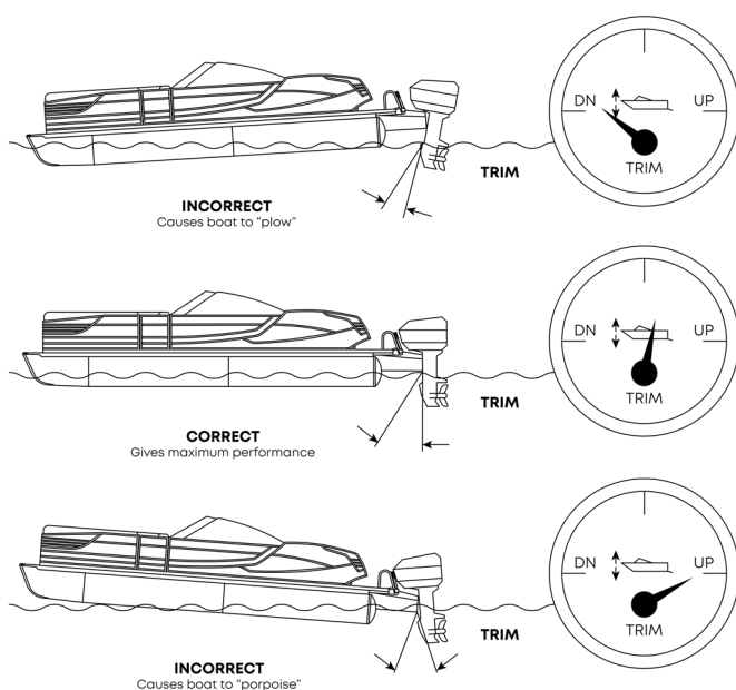
FIGURE 5-4 TRIMMING
