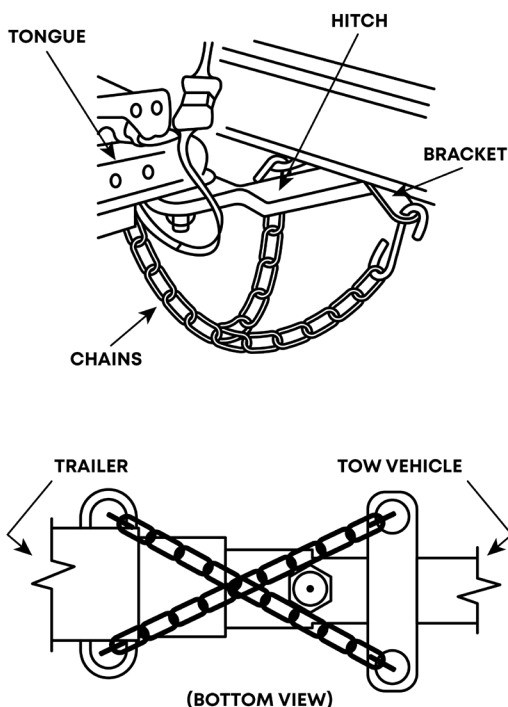
FIGURE 4-1 SAFETY CHAINS
