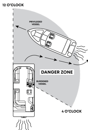
FIGURE 8-2 CROSSING
